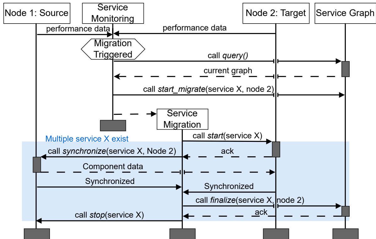
Figure 3.3: Polka service migration message sequence chart.
